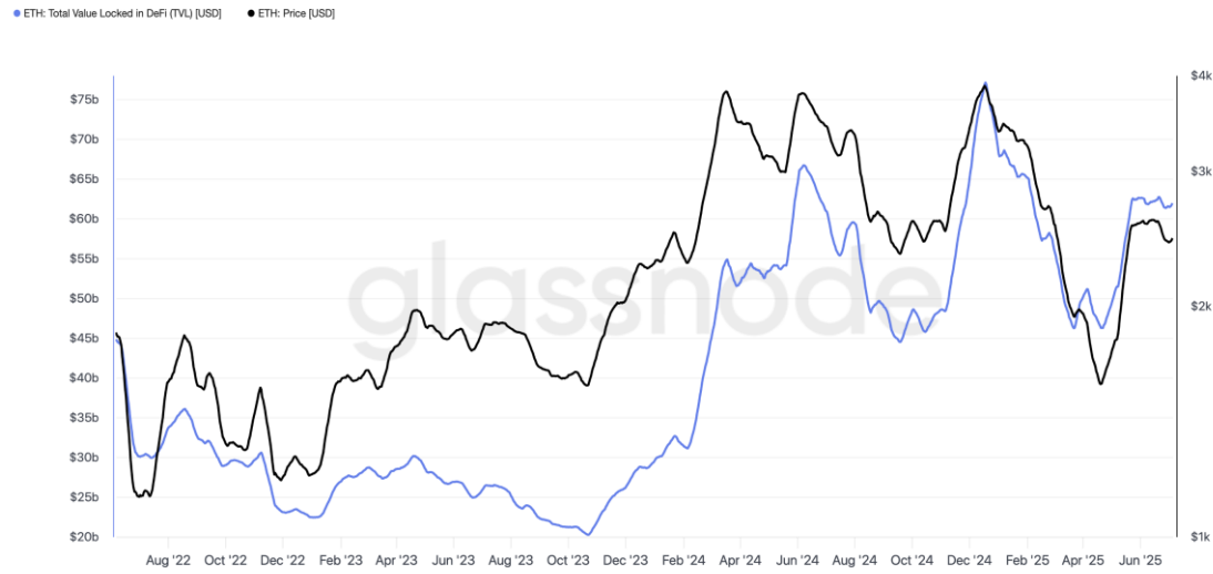
ETH: Total Value Locked in DeFi (TVL)
